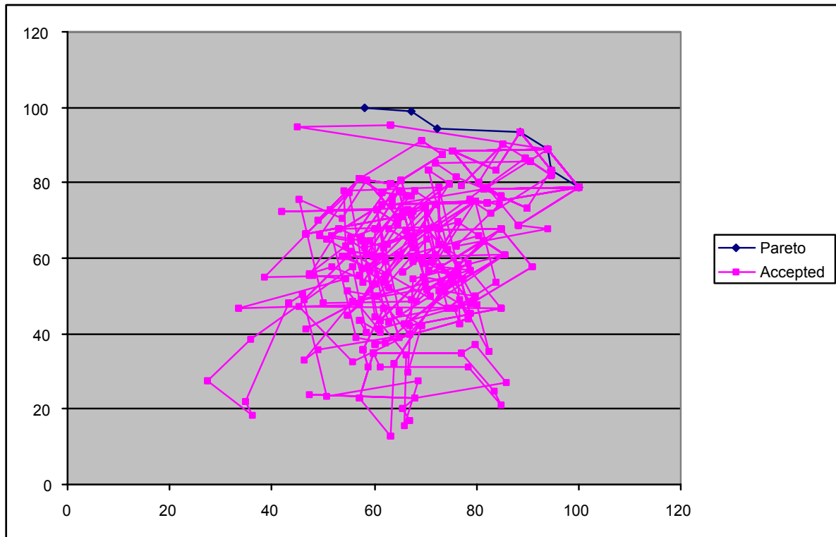
Figure 6: A typical negotiation with two annealers.
