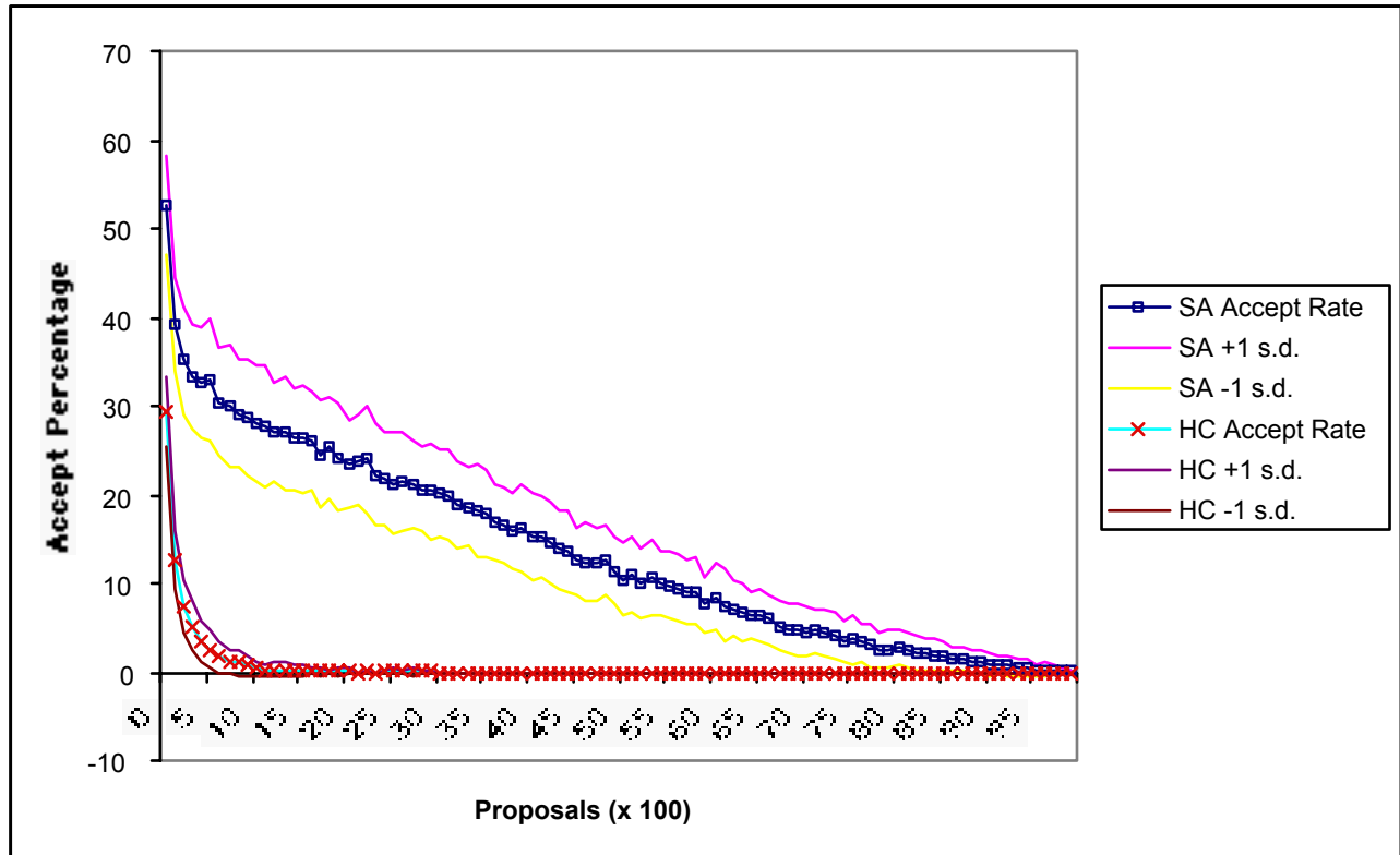
Figure 4: Proposal acceptance percentages for hill-climbers and annealers.
