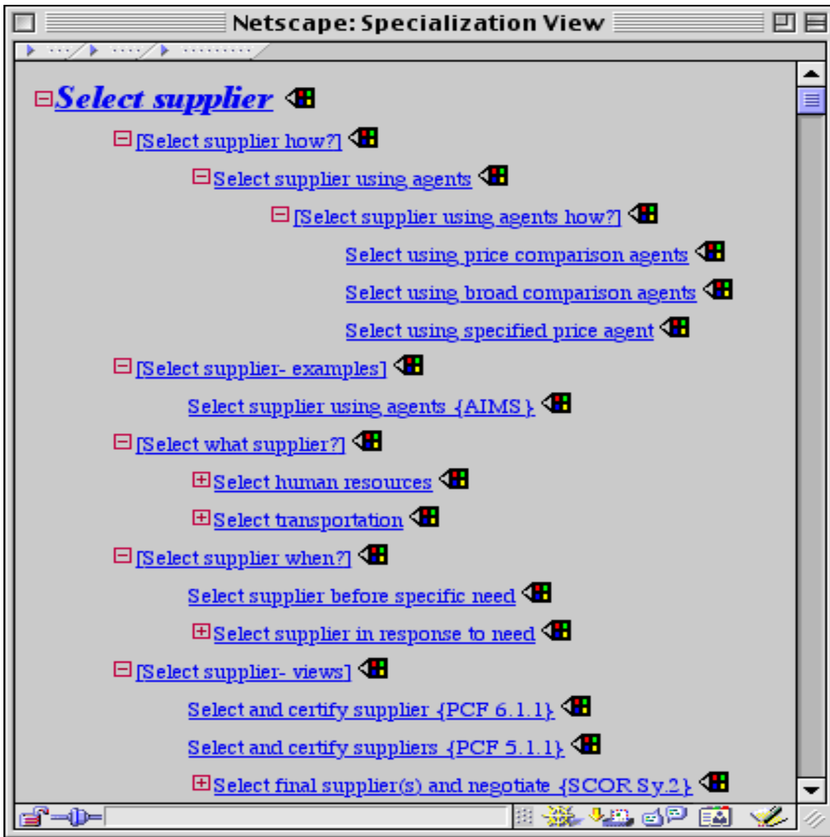
Figure 7: A fragment of the ‘select supplier’ ontology.
