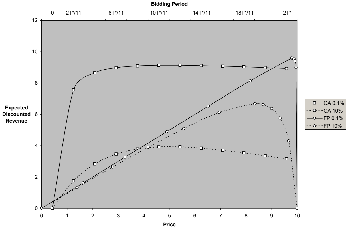
Figure 1: E[FP(p)] and E[OA(T)] for K = 1 and \beta \in \{0.1\%, 10\%\} .
