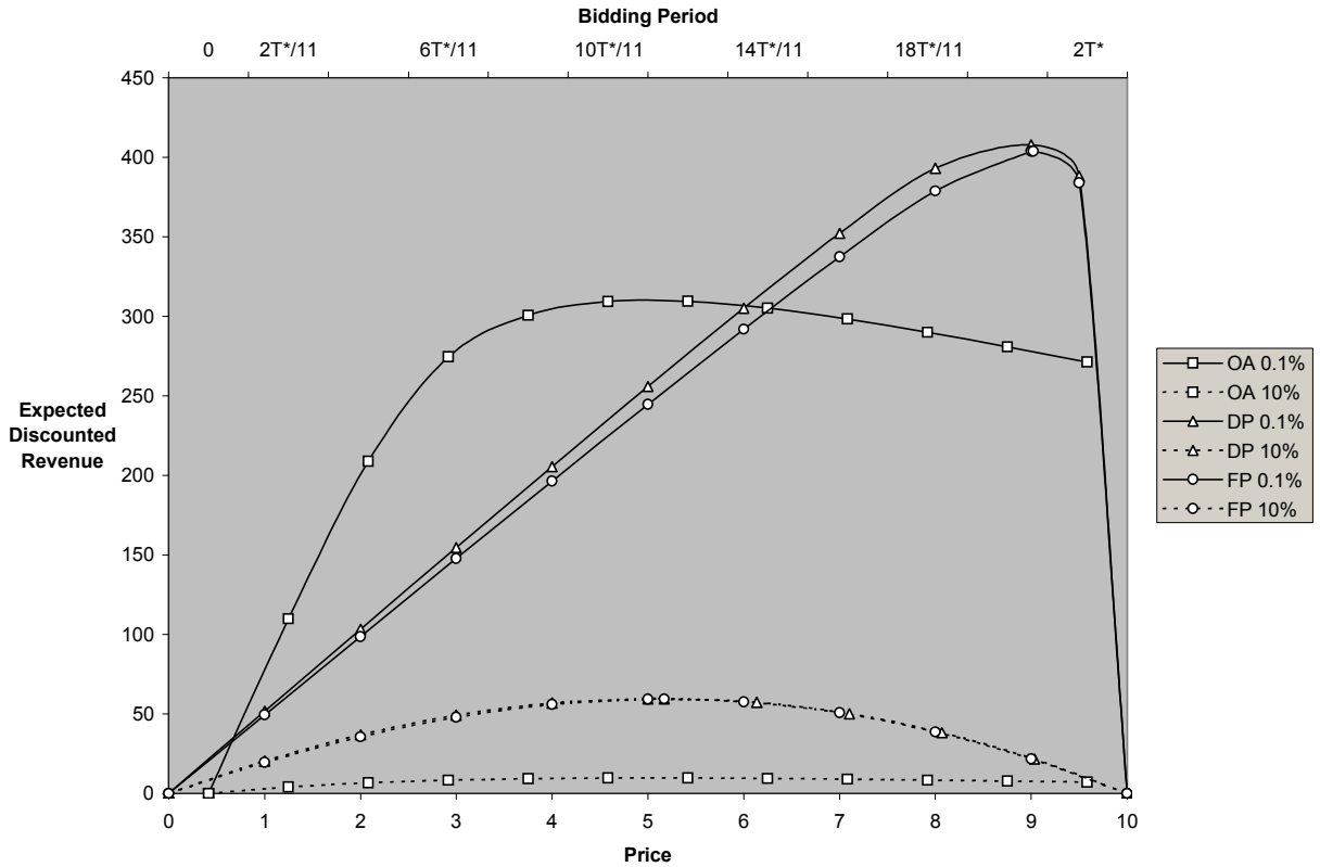
Figure 2: E[DP((p_k(p))_{k \leq K})] , E[FP(p)] and E[OA(T)] for K = 50 and \beta \in \{0.1\%, 10\%\} .
